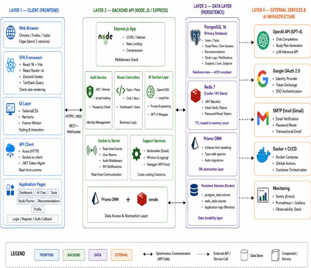
Figure: System Architecture Diagram of the AI-Based Smart Learning Assistant
